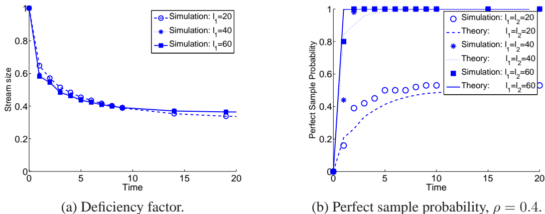
Figure 9: Dynamics within a targeted node ( n = 1000, p = 0.2, \alpha = \beta = 0.5 and \gamma = 0 ): (a) Fraction of unique ids in the stream of correct ids, which is an upper bound on the deficiency factor \rho . (b) Growth of Perfect Sample Probability (PSP) with time, \rho = 0.4 . PSP becomes high quickly enough to prevent isolation.
