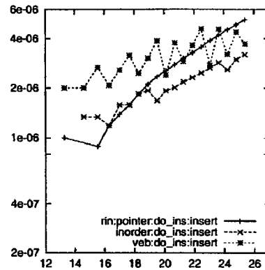
Figure 6: Insert time per element
