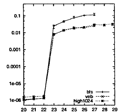
Figure 8: Beyond main memory
