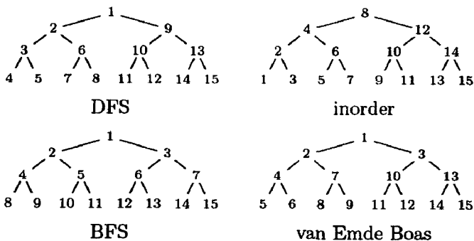
Figure 2: The DFS, inorder, BFS, and van Emde Boas layouts for a complete tree with height 4. Numbers designate positions in the array of node records
