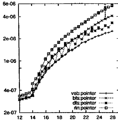
Figure 3: Searches for pointer based layouts
