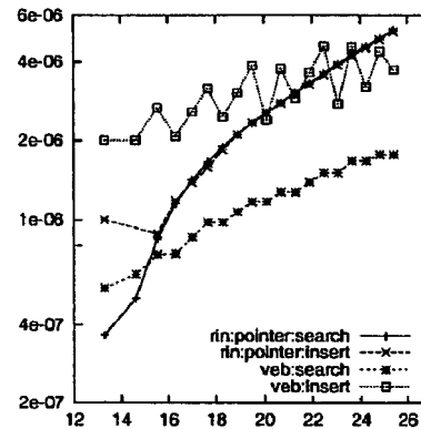
Figure 7: Insert and Search for implicit veb and unbalanced search trees
