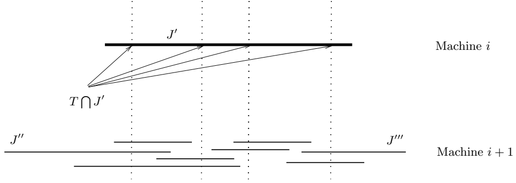
Figure 3: Analysis of a job J' assigned to machine M_i
