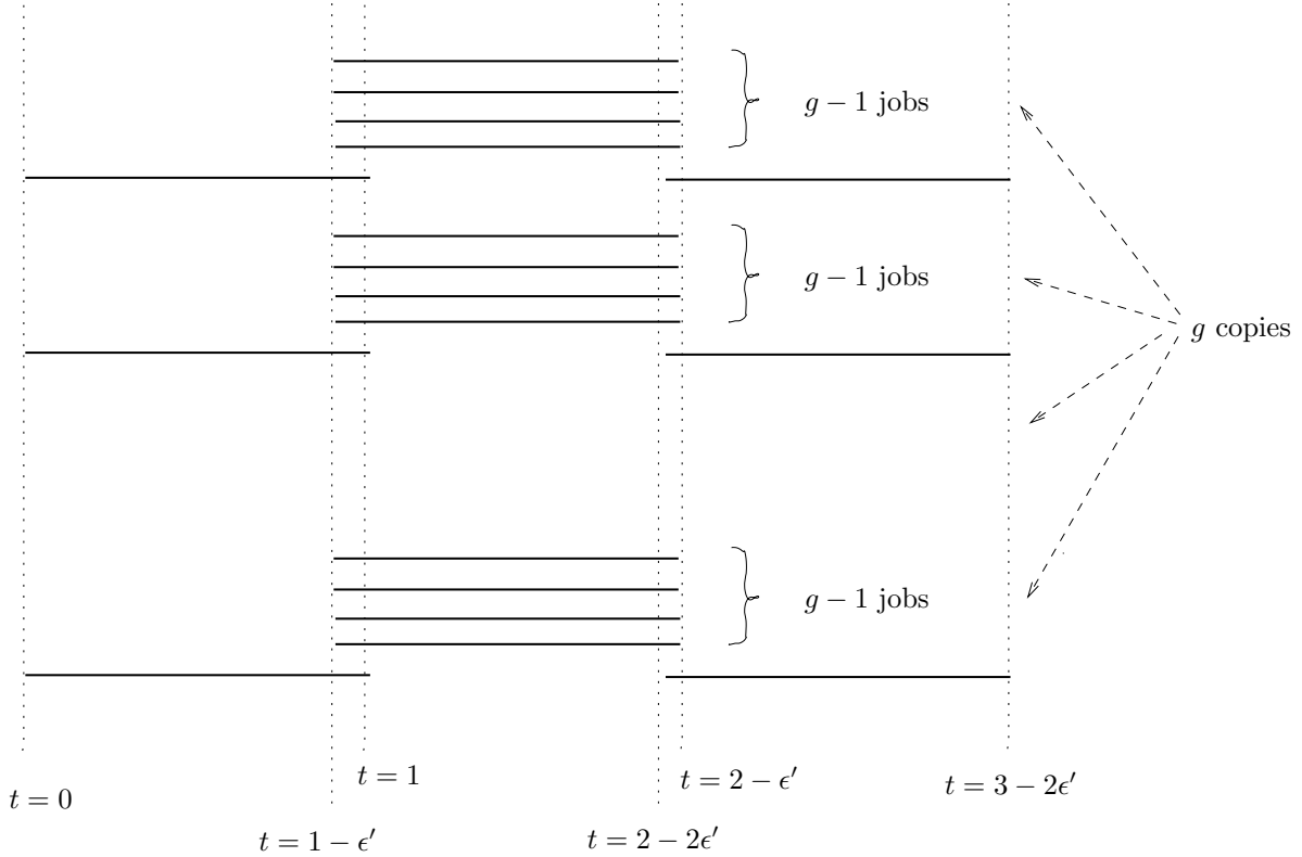
Figure 4: Instance for the proof of the lower bound
