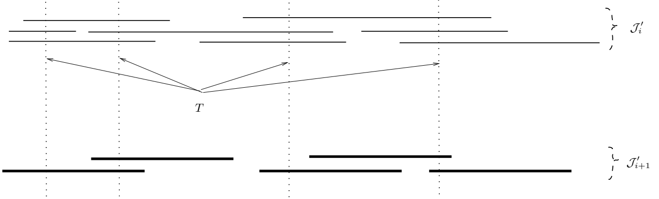
Figure 2: Lemma 2.3 setting
