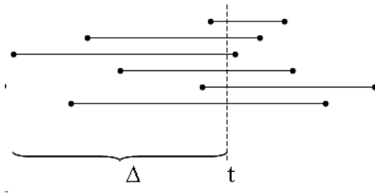
Figure 5: The left-right partition of a clique for an arbitrary intersection point t .
