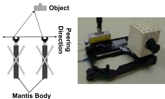
Figure 3.1: Scheme of Peering Behavior of Praying Mantis and the implementation of the Miniature Mantis Head Camera Platform, which utilizes peering behavior for distance estimation
